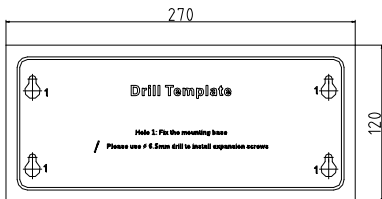
Figure 2-7 Drill Template
