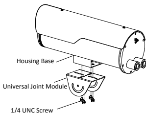
Figure 2-3 Install the Universal Joint Module
