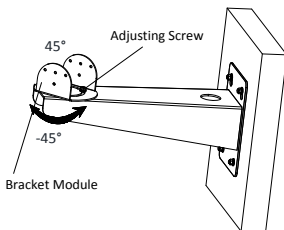
Figure 2-4 Adjust the Surveillance Angle
