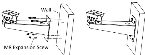
Figure 2-1 Install the Bracket
