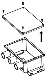
Figure 2-8 Open the Junction Box
