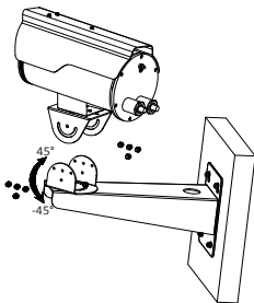
Figure 2-5 Install the Housing onto Bracket
