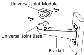
Figure 2-2 Take Off the Bracket
