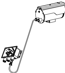
Figure 2-10 Route the Cables
