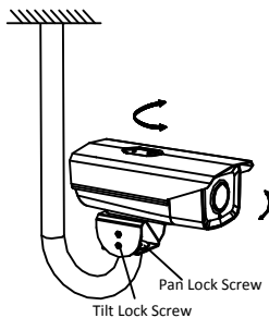
Figure 2-8 Adjust Surveillance Angle
