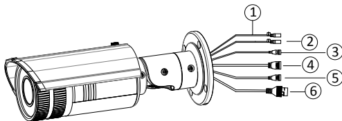
Figure 1-3 Wiring (B)
