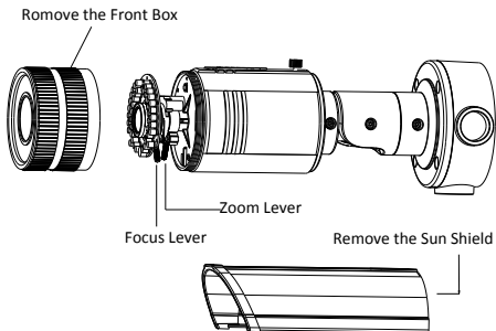
Figure 2-5 Lens Adjustment
