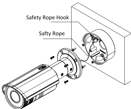
Figure 2-3 Fix the Camera to the Junction Box
