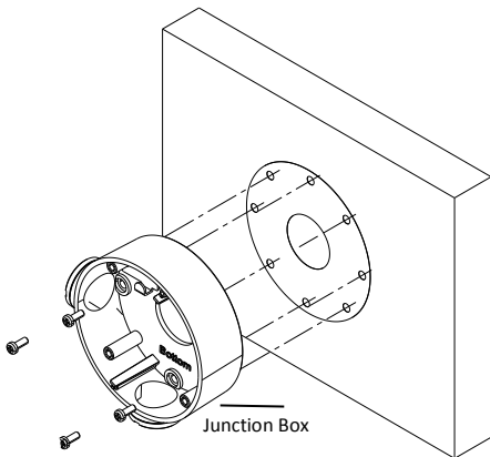
Figure 2-2 Install the Junction Box
