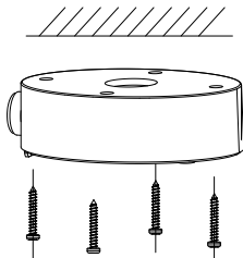
Figure 2-2 Install Junction Box
