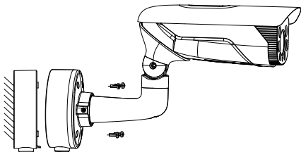
Figure 2-7 Install Camera
