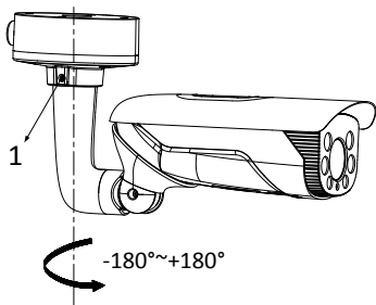
Figure 2-9 Adjust Pan Angle
