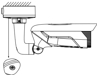
Figure 2-4 Tighten the Lock Screw
