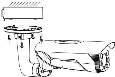
Figure 2-3 Install Camera
