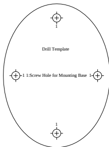
Figure 2-1 Drill Template
