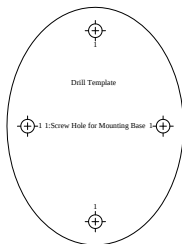
Figure 2-5 Drill Template
