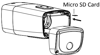
Figure 2-7 Install the Micro SD Card
