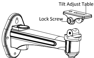
Figure 2-1 Remove the Tilt Adjust Table
