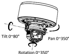
Figure 2-4 3-axis Adjustment
