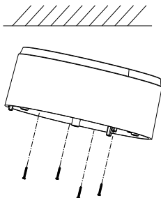
Figure 2-9 Install the Mounting Base
