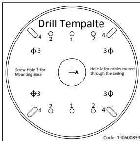
Figure 2-1 Drill Template
