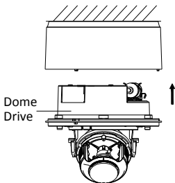
Figure 2-3 Install the Dome Drive
