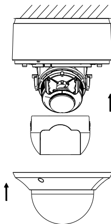
Figure 2-6 Install the Black Liner and Bubble
