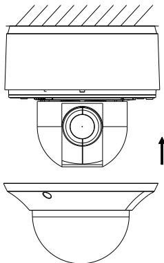
Figure 2-12 Install the Bubble
