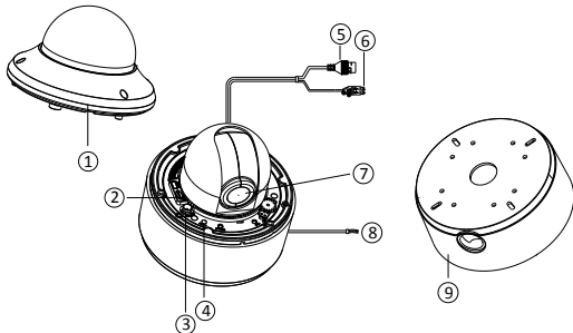
Figure 1-3 Overview of Type II Dome Camera
