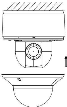
Figure 2-10 Install the Dome Drive
