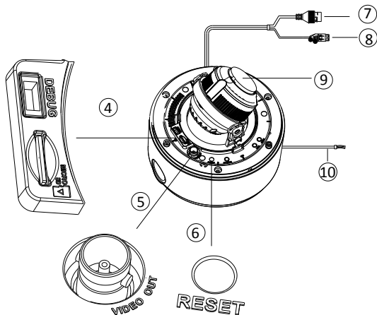
Figure 1-2 Overview (2) of Type II Dome Camera
