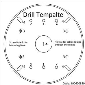
Figure 2-8 Drill Template
