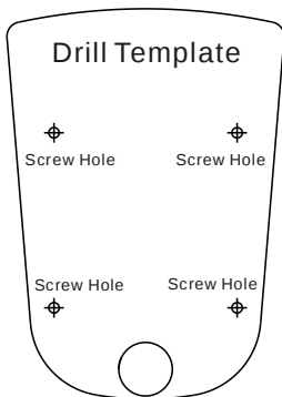
Figure 2-1 Drill Template
