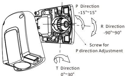
Figure 2-6 3-axis Adjustment
