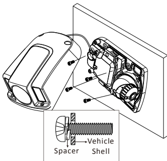
Figure 2-3 Fit the Mounting Screws
