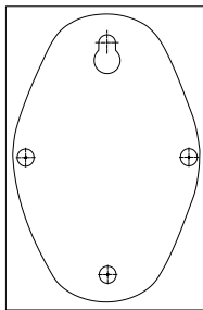
Figure 2-1 Drill Template
