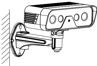
Figure 2-5 Secure the Camera to the Wall Bracket
