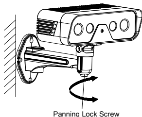
Figure 2-6 Adjust Panning Angle
