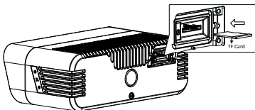
Figure 2-13 Insert the TF Card
