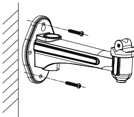
Figure 2-3 Install the Wall Bracket
